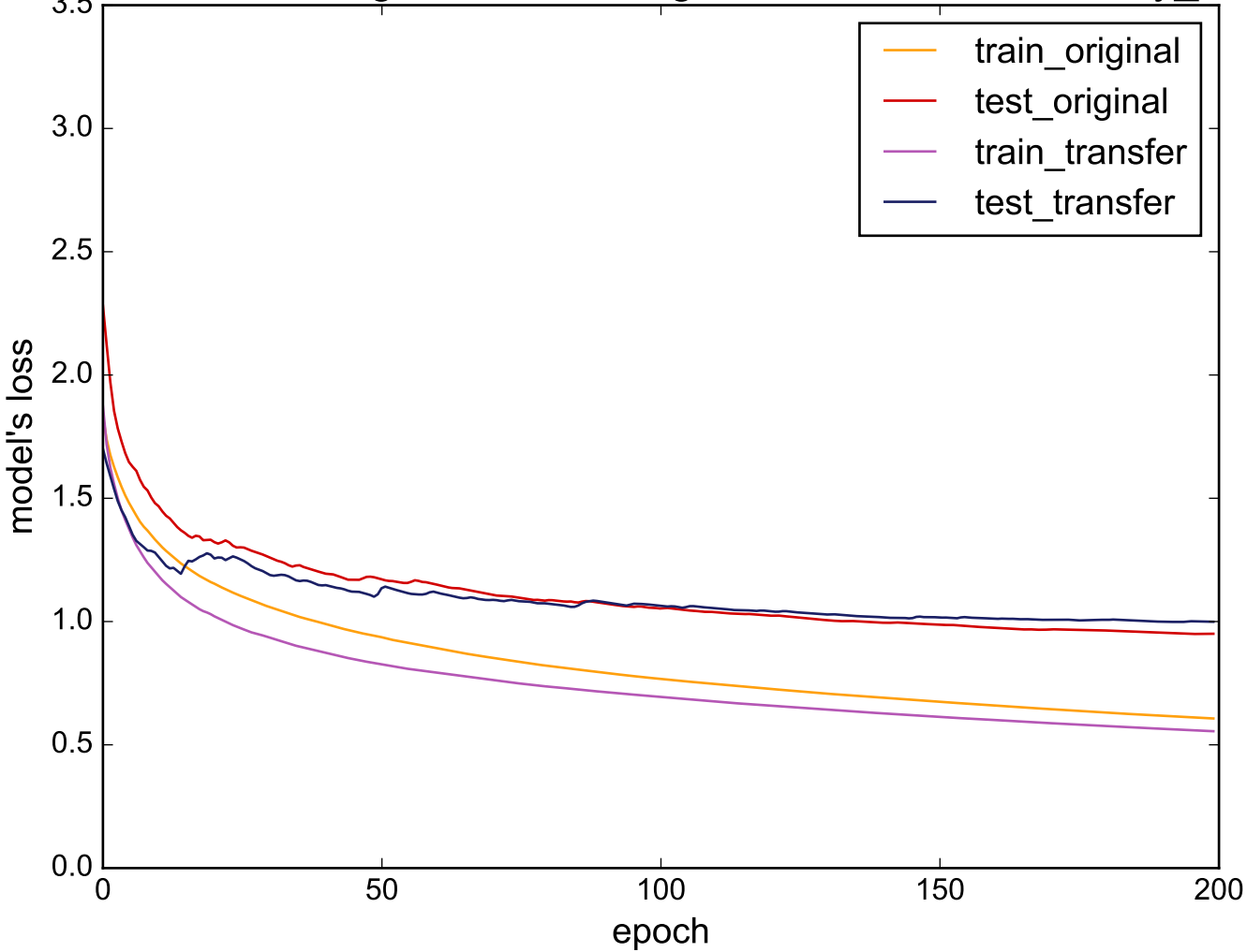
Source: StarLightCurves - Target: uWaveGestureLibrary_X
