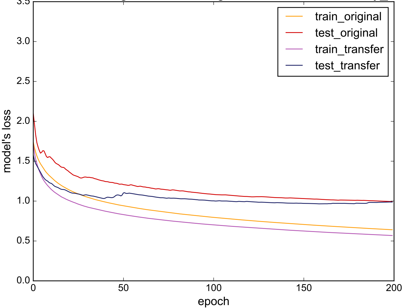
Source: StarLightCurves - Target: uWaveGestureLibrary_Z
