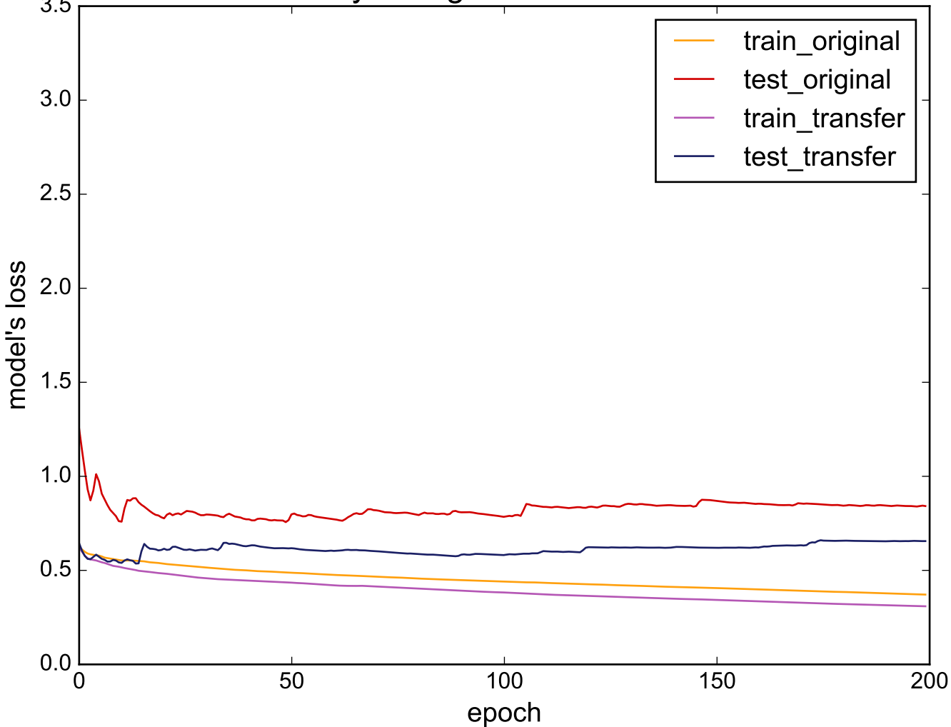
Source: Strawberry - Target: DistalPhalanxOutlineCorrect
