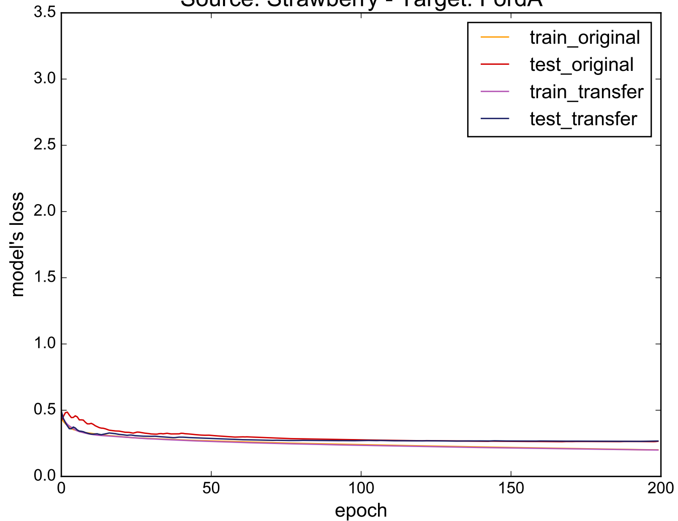
Source: Strawberry - Target: FordA
