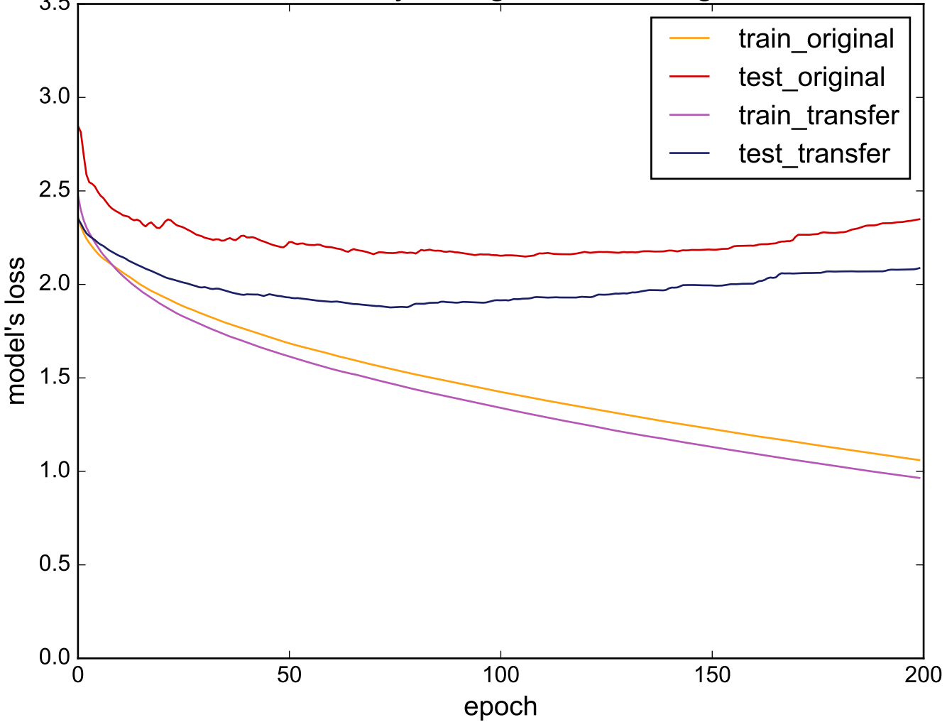
Source: Strawberry - Target: InsectWingbeatSound
