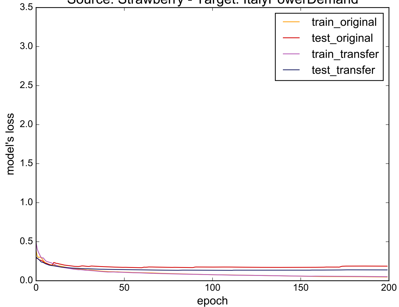
Source: Strawberry - Target: ItalyPowerDemand
