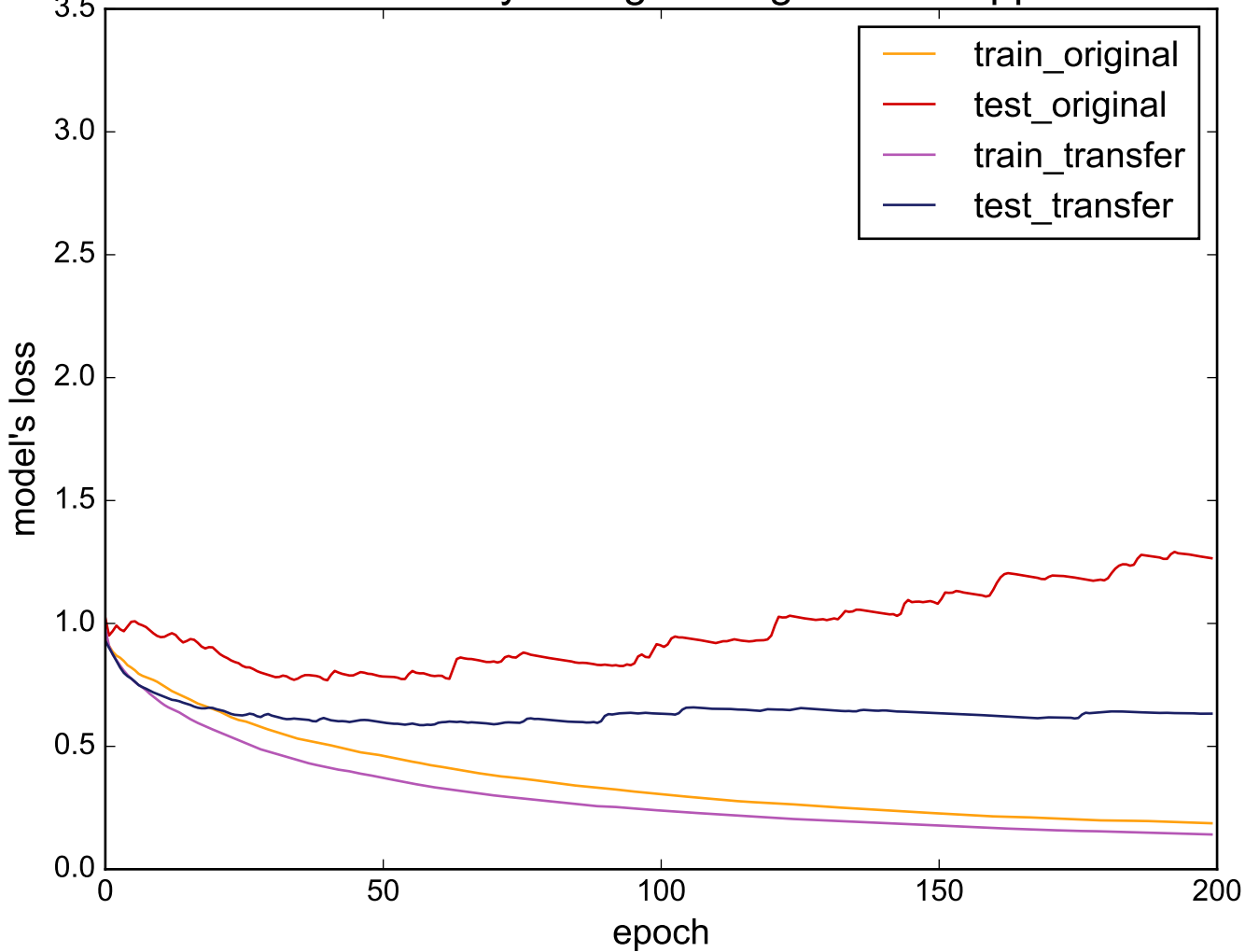
Source: Strawberry - Target: LargeKitchenAppliances
