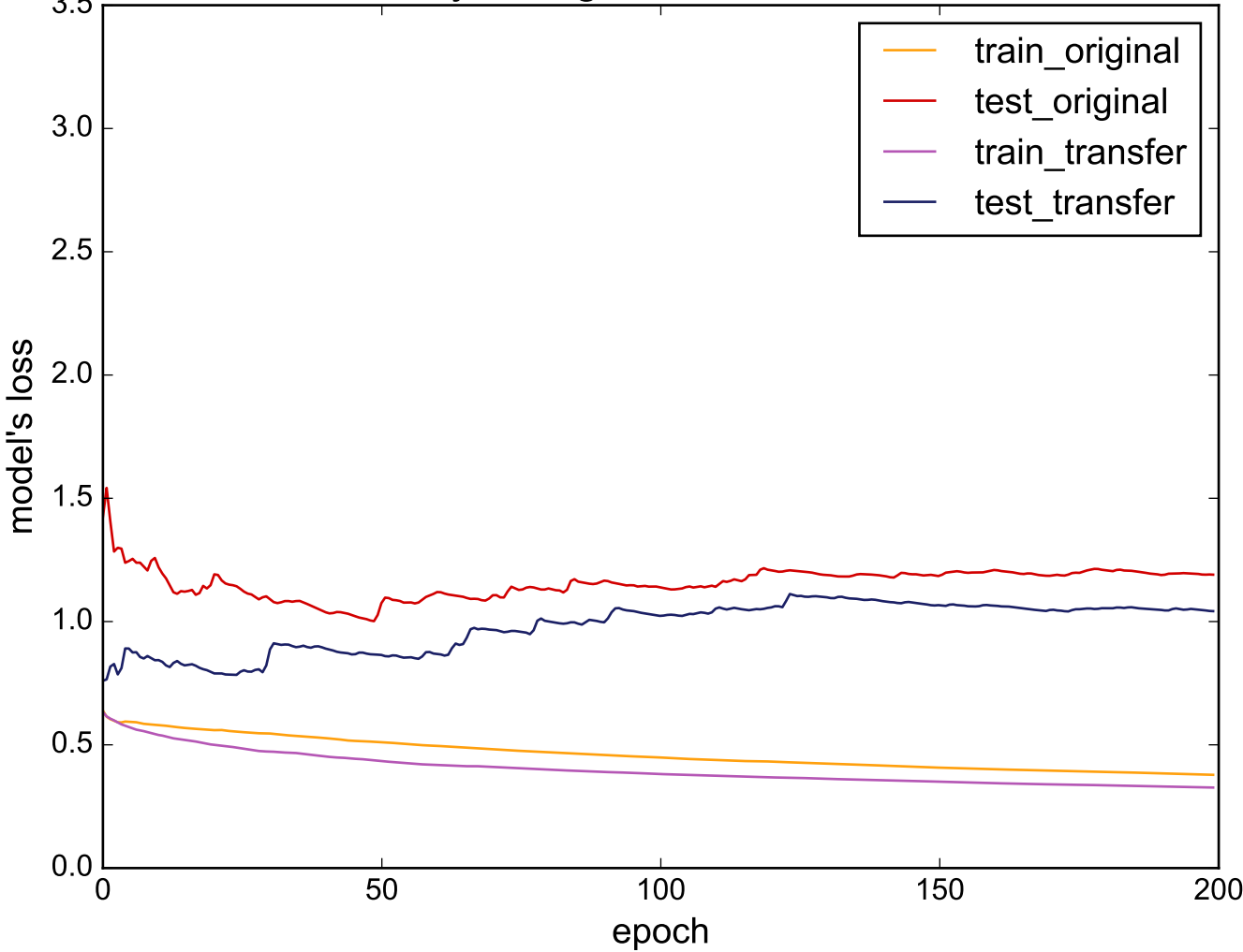
Source: Strawberry - Target: MiddlePhalanxOutlineCorrect
