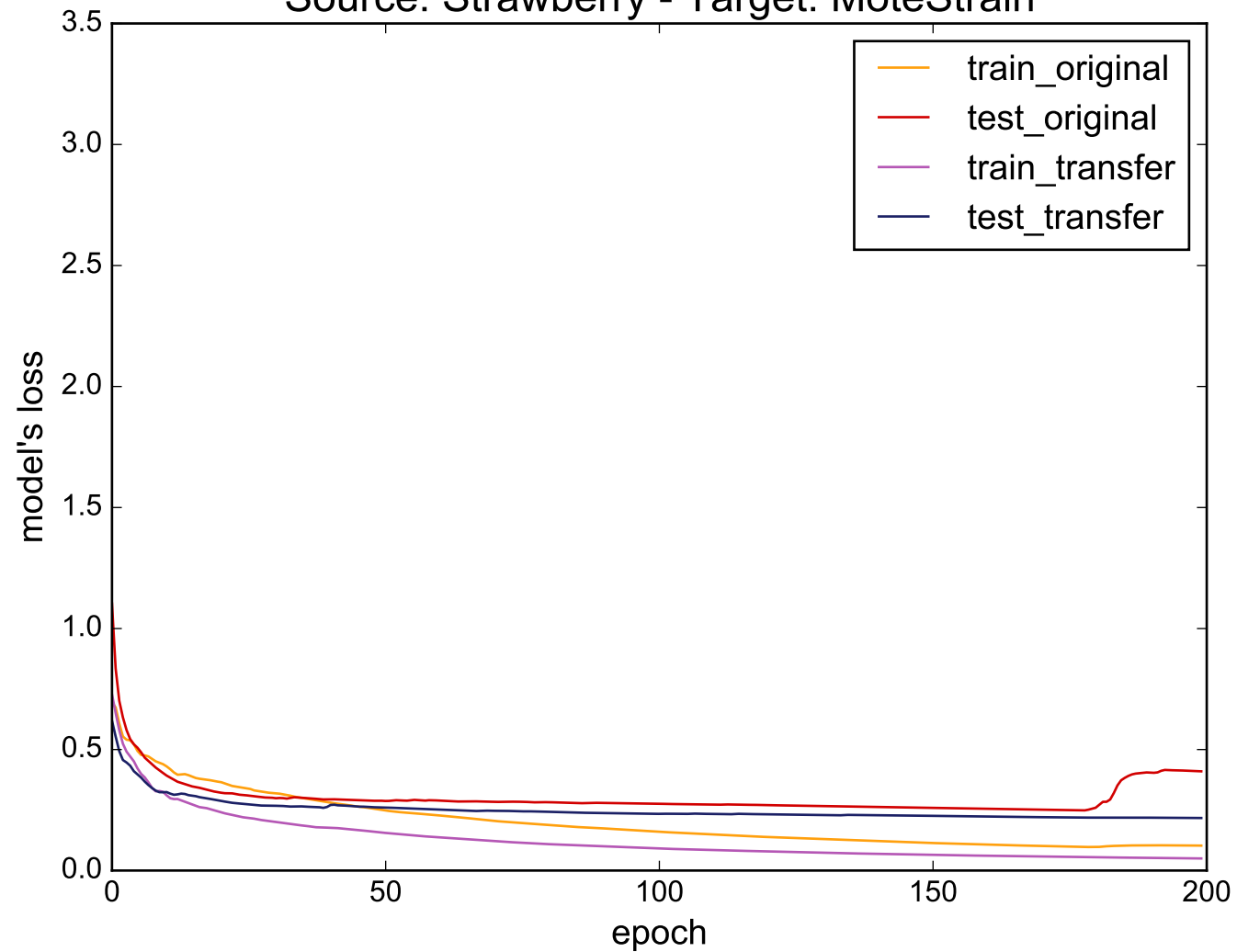
Source: Strawberry - Target: MoteStrain
