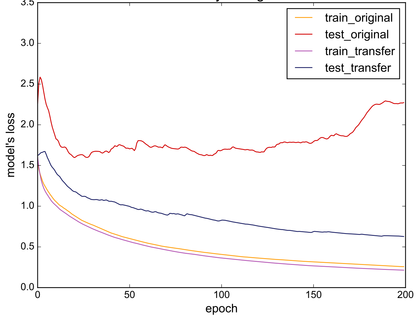
Source: Strawberry - Target: OSULeaf
