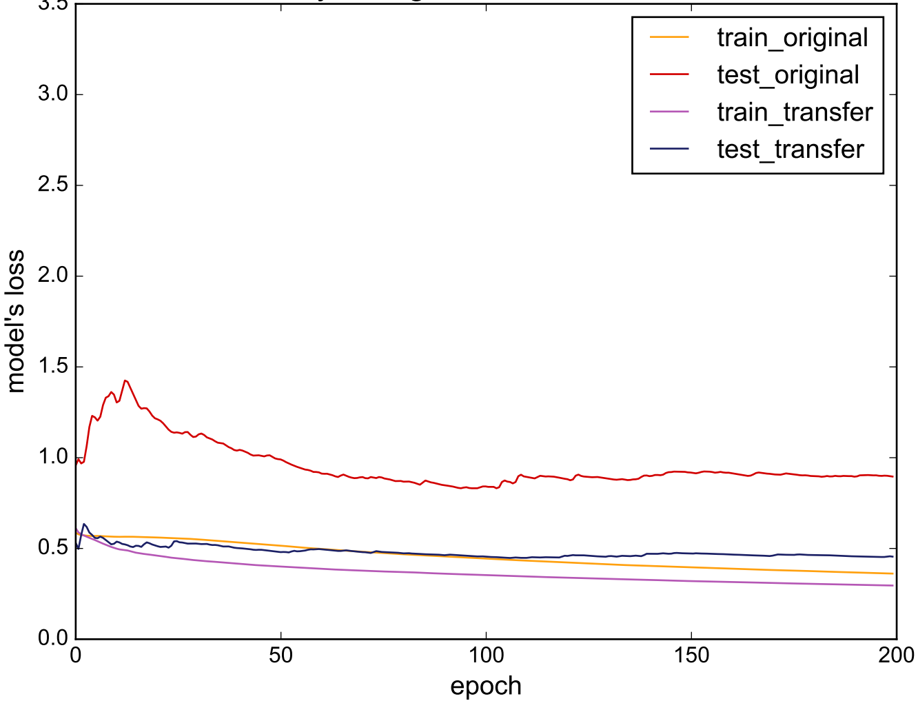
Source: Strawberry - Target: ProximalPhalanxOutlineCorrect
