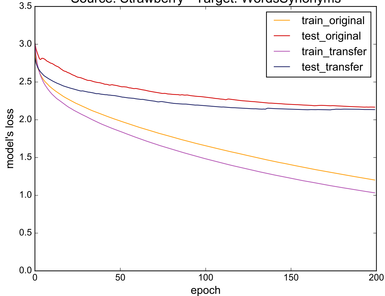
Source: Strawberry - Target: WordsSynonyms
