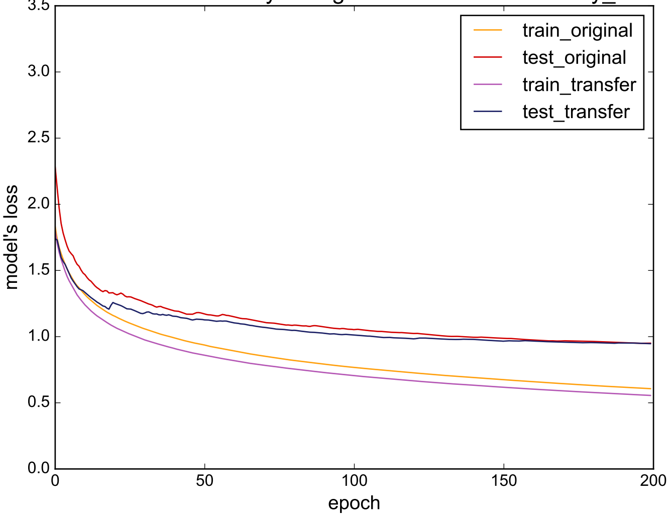
Source: Strawberry - Target: uWaveGestureLibrary_X
