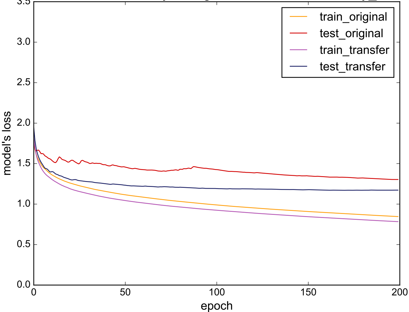
Source: Strawberry - Target: uWaveGestureLibrary_Y
