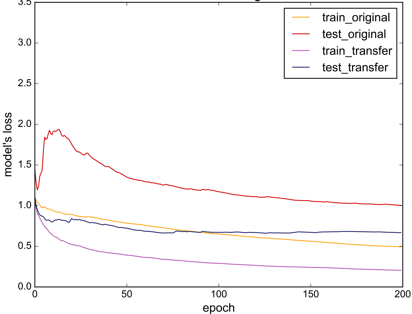
Source: SwedishLeaf - Target: ArrowHead
