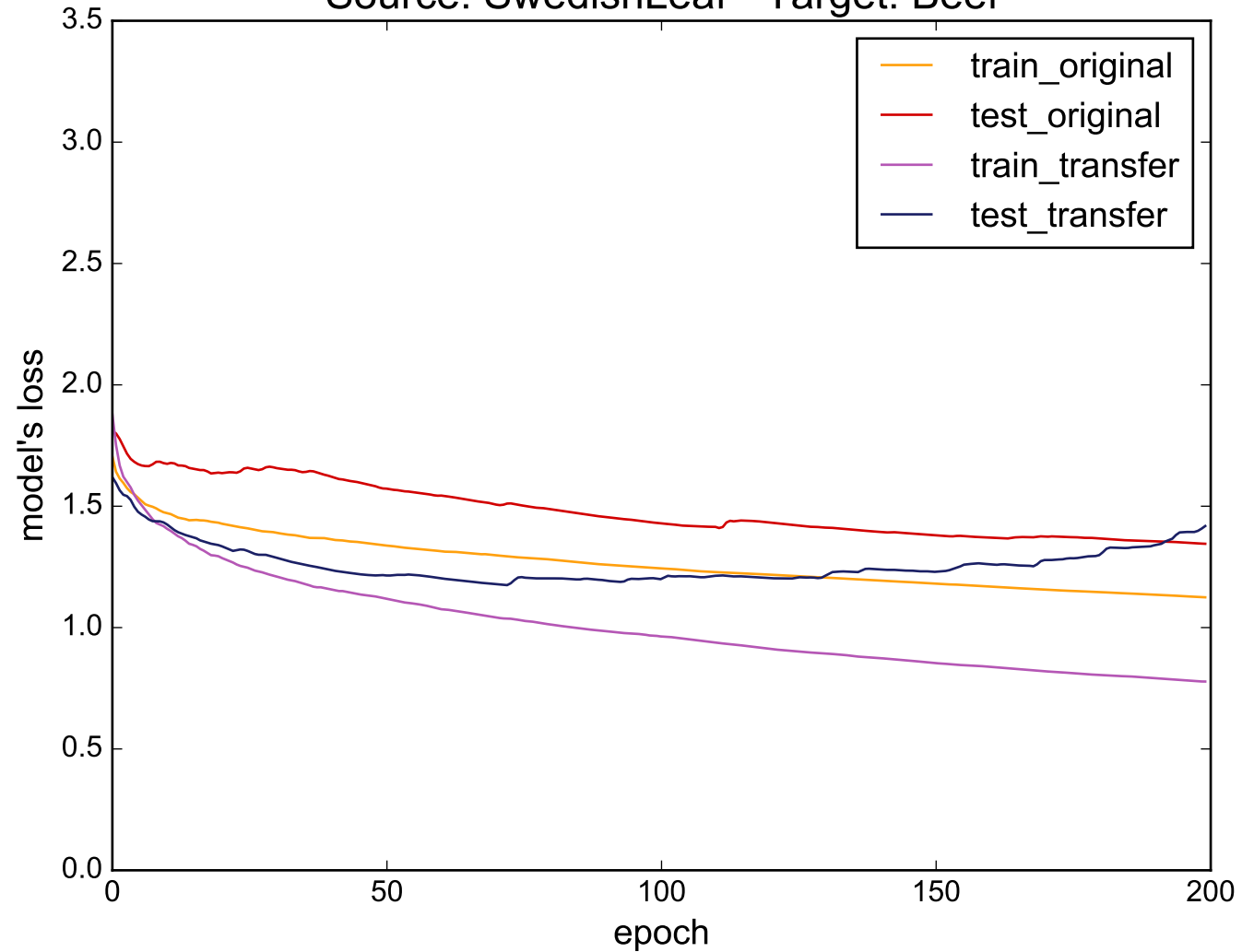
Source: SwedishLeaf - Target: Beef
