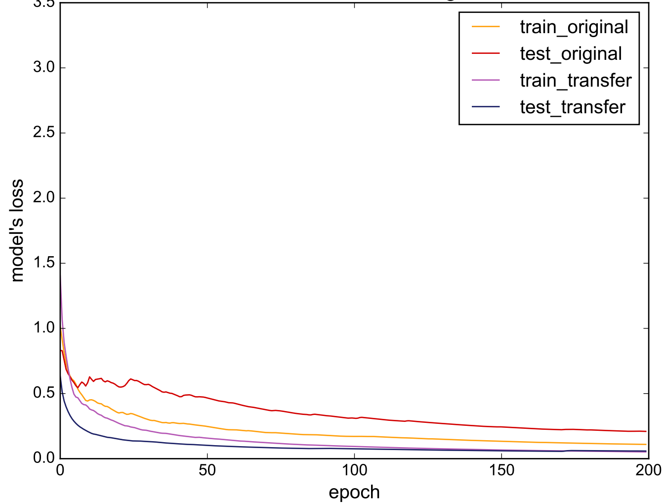
Source: SwedishLeaf - Target: CBF
