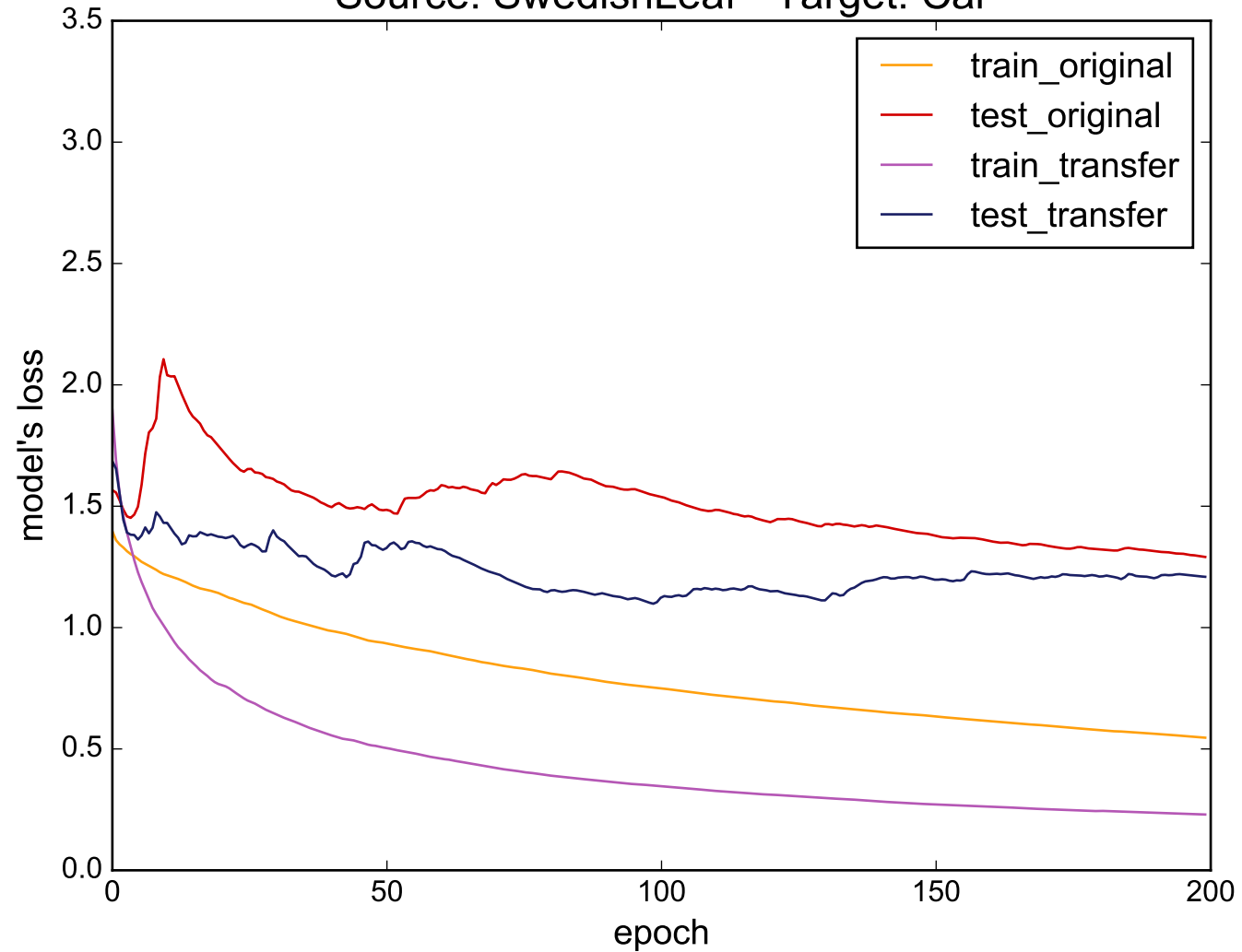
Source: SwedishLeaf - Target: Car
