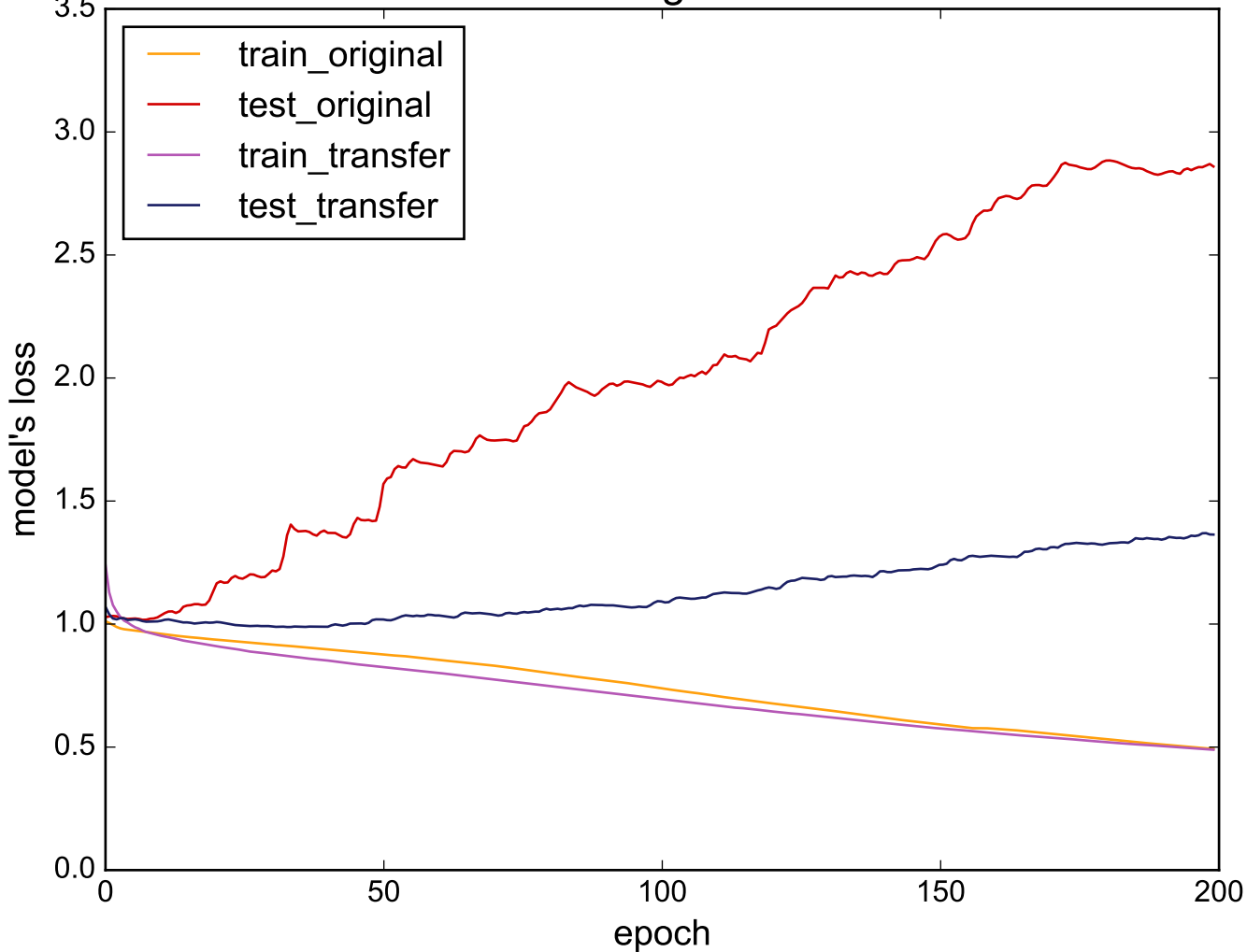
Source: SwedishLeaf - Target: ChlorineConcentration
