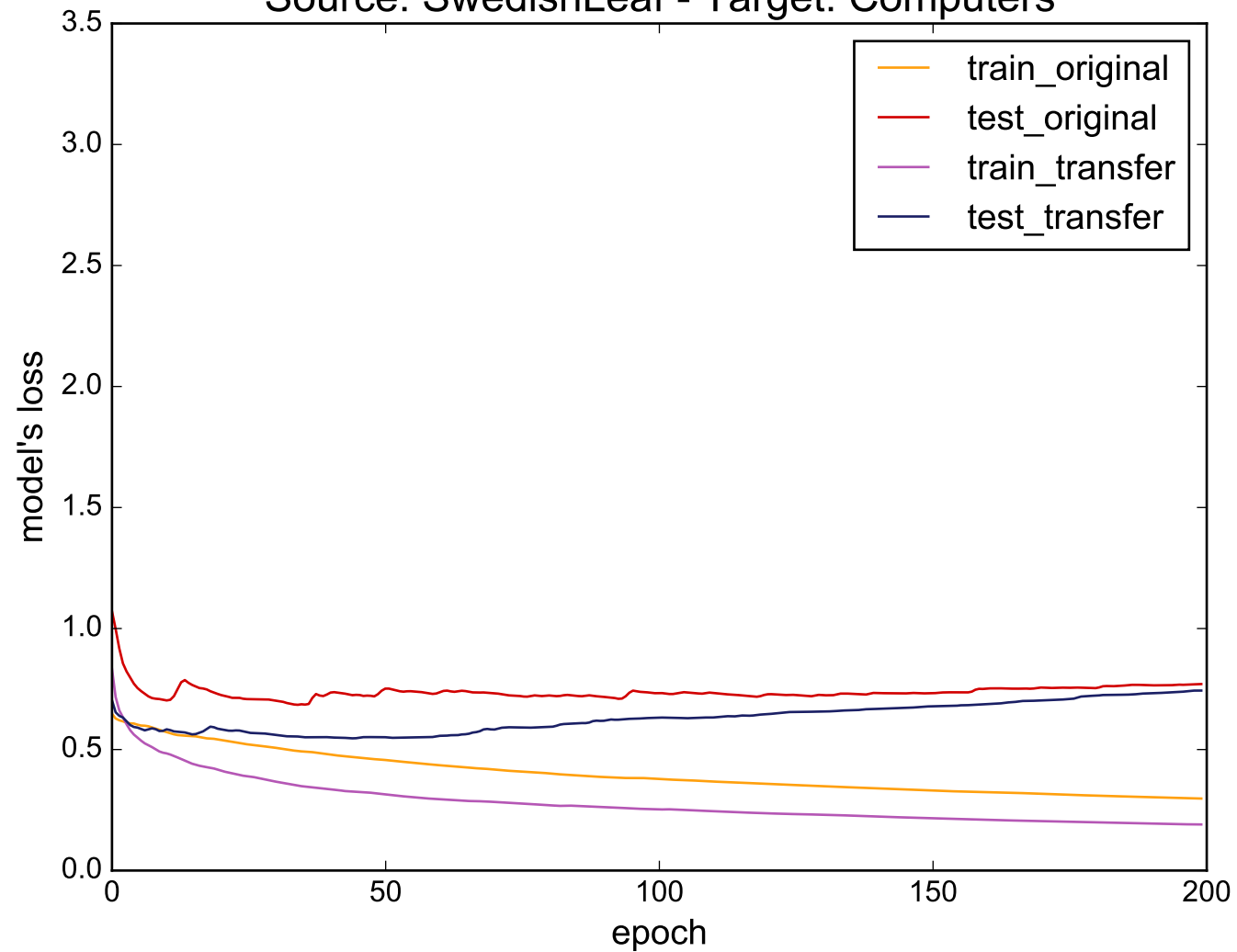
Source: SwedishLeaf - Target: Computers
