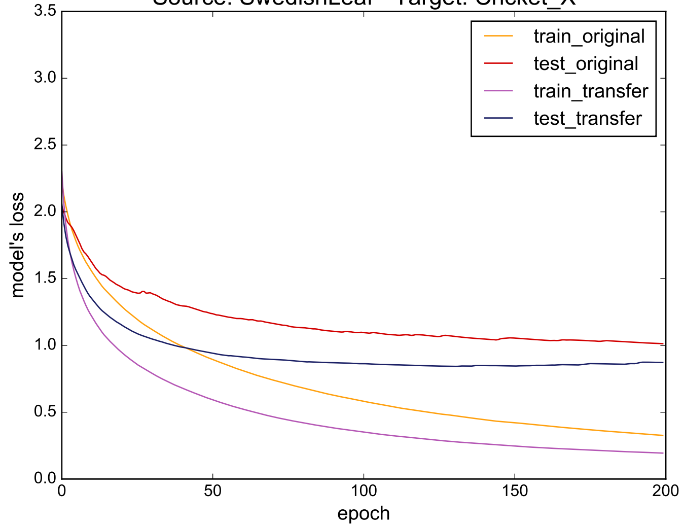
Source: SwedishLeaf - Target: Cricket_X
