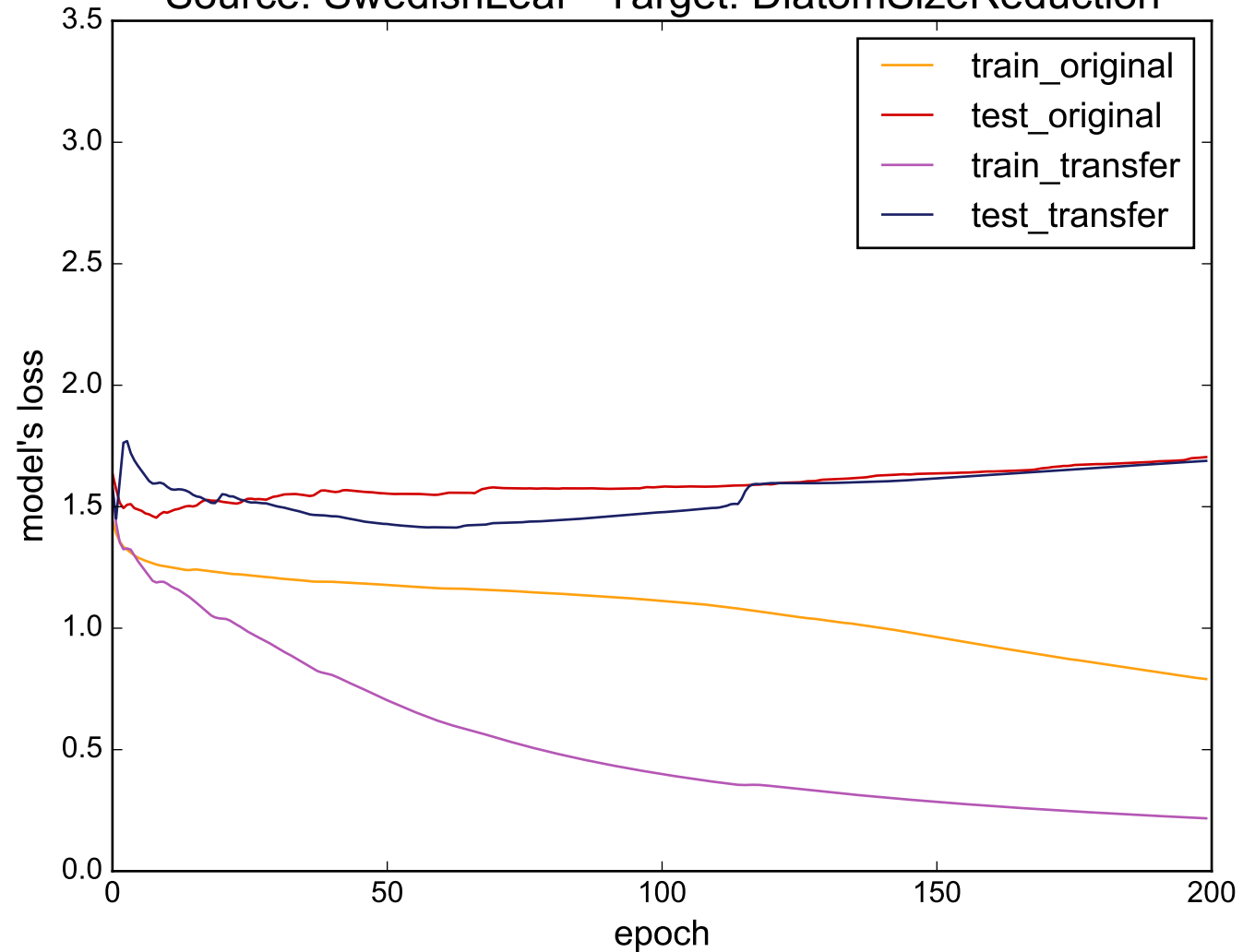
Source: SwedishLeaf - Target: DiatomSizeReduction
