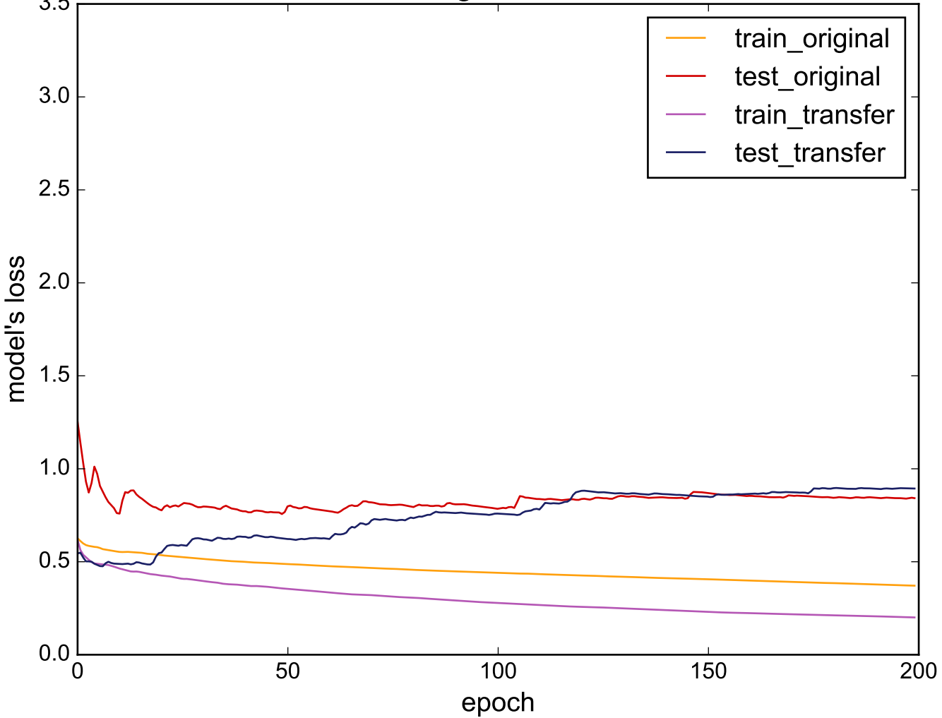
Source: SwedishLeaf - Target: DistalPhalanxOutlineCorrect
