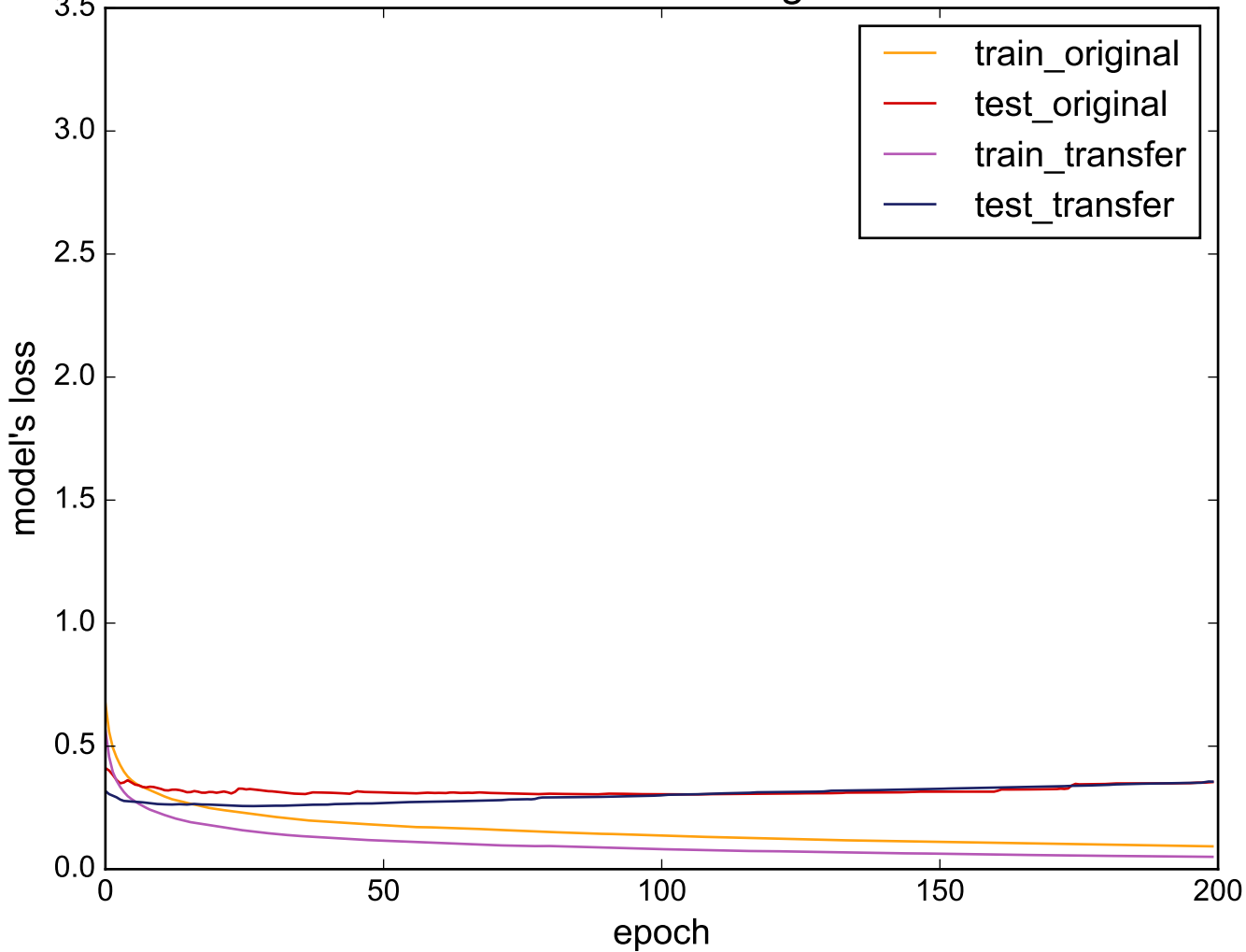
Source: SwedishLeaf - Target: ECG5000
