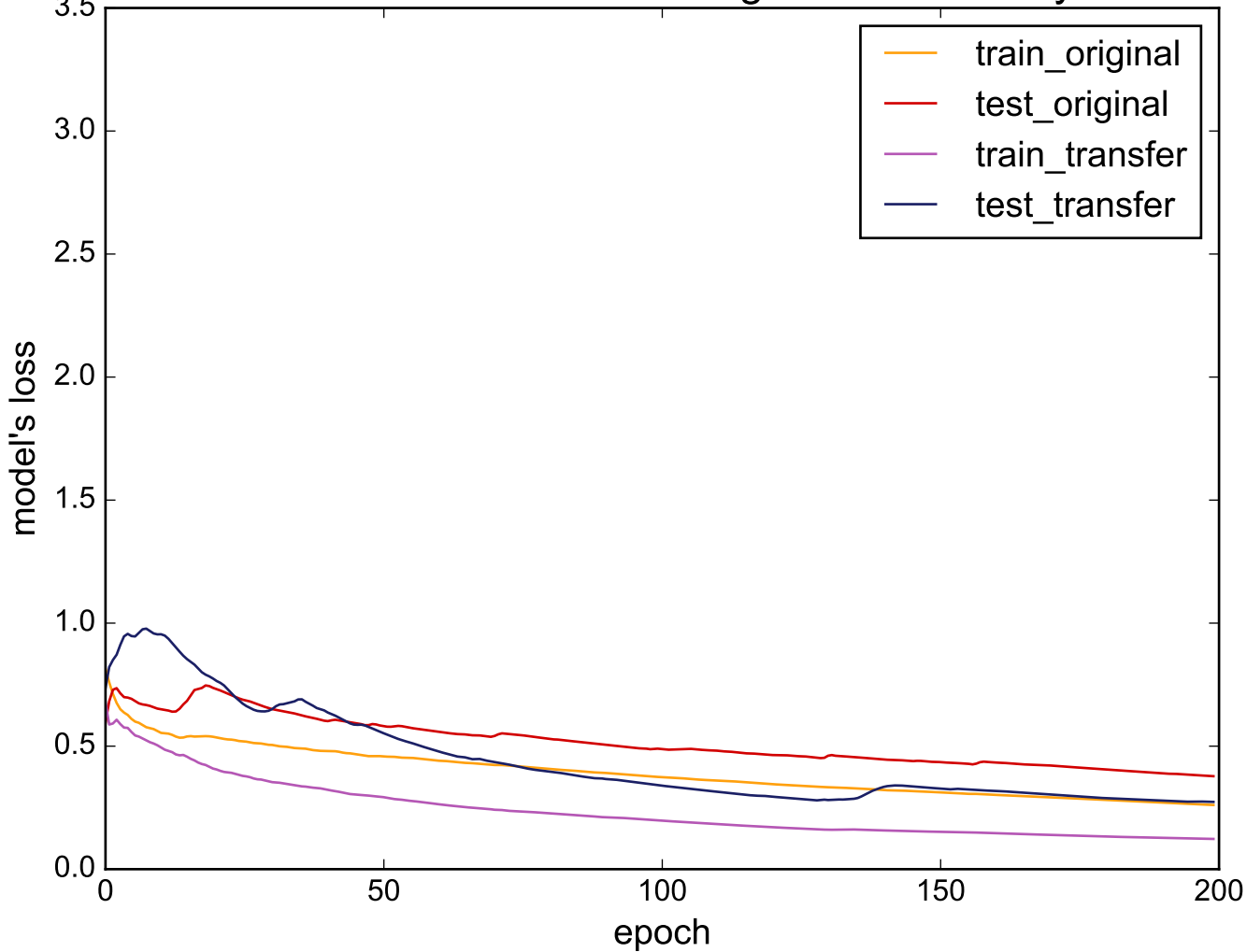
Source: SwedishLeaf - Target: ECGFiveDays
