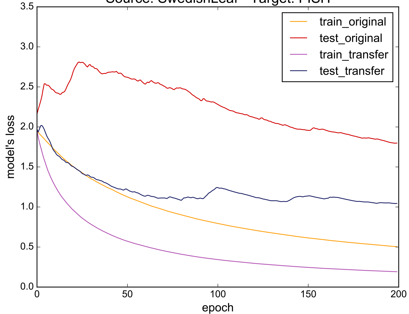
Source: SwedishLeaf - Target: FISH
