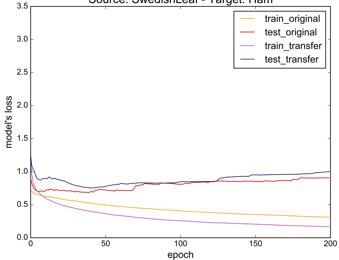
Source: SwedishLeaf - Target: Ham
