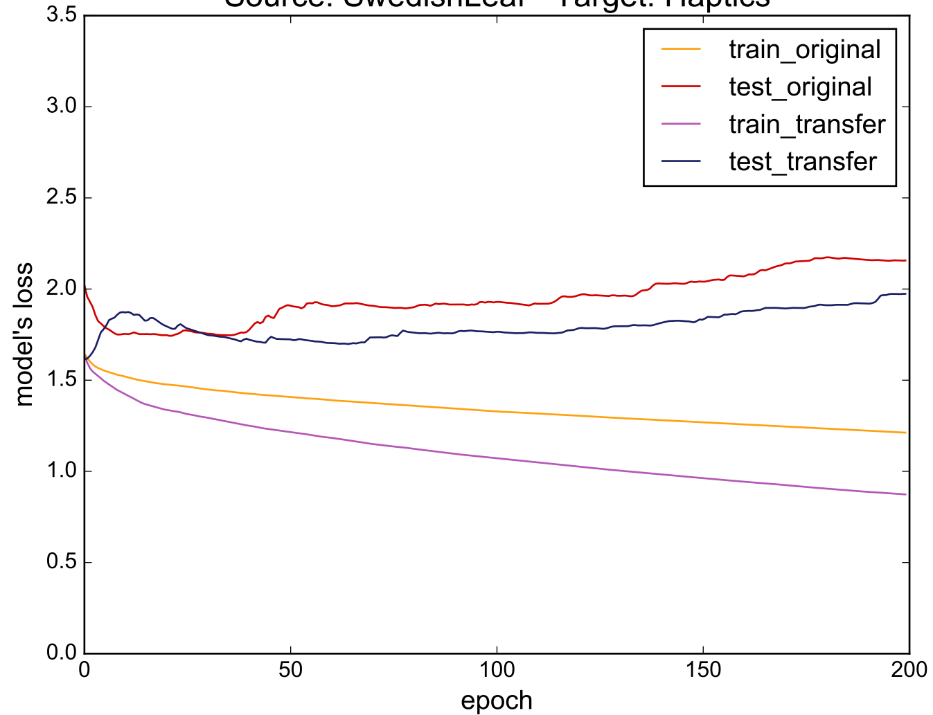
Source: SwedishLeaf - Target: Haptics
