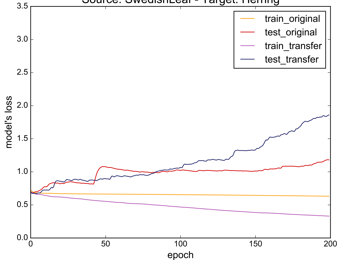
Source: SwedishLeaf - Target: Herring
