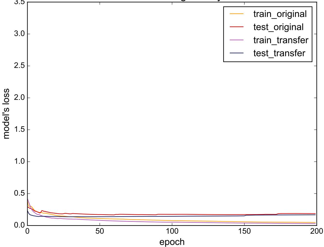
Source: SwedishLeaf - Target: ItalyPowerDemand
