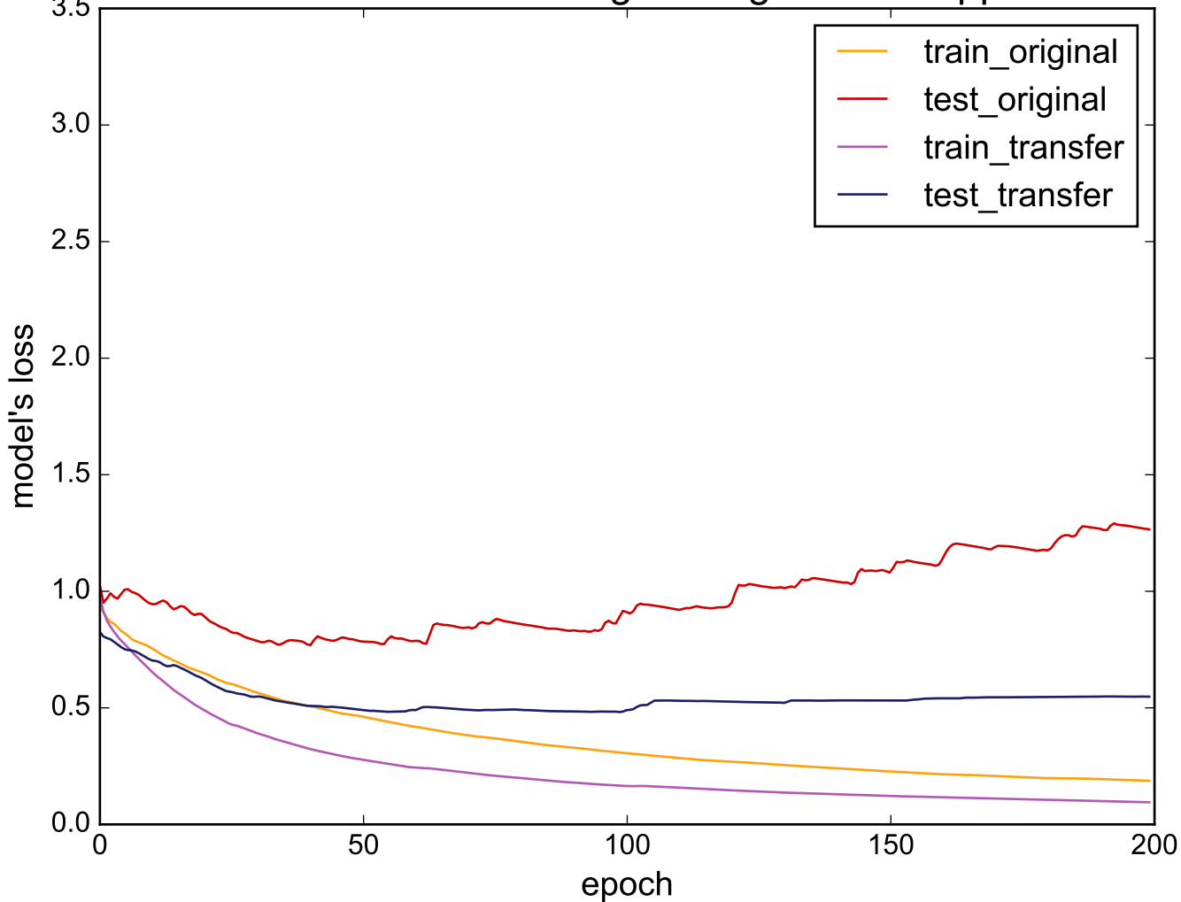
Source: SwedishLeaf - Target: LargeKitchenAppliances
