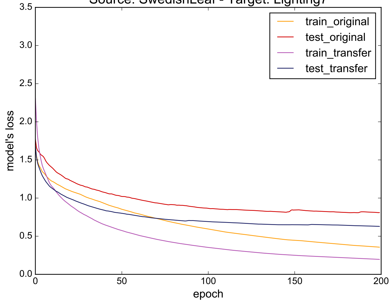
Source: SwedishLeaf - Target: Lighting7
