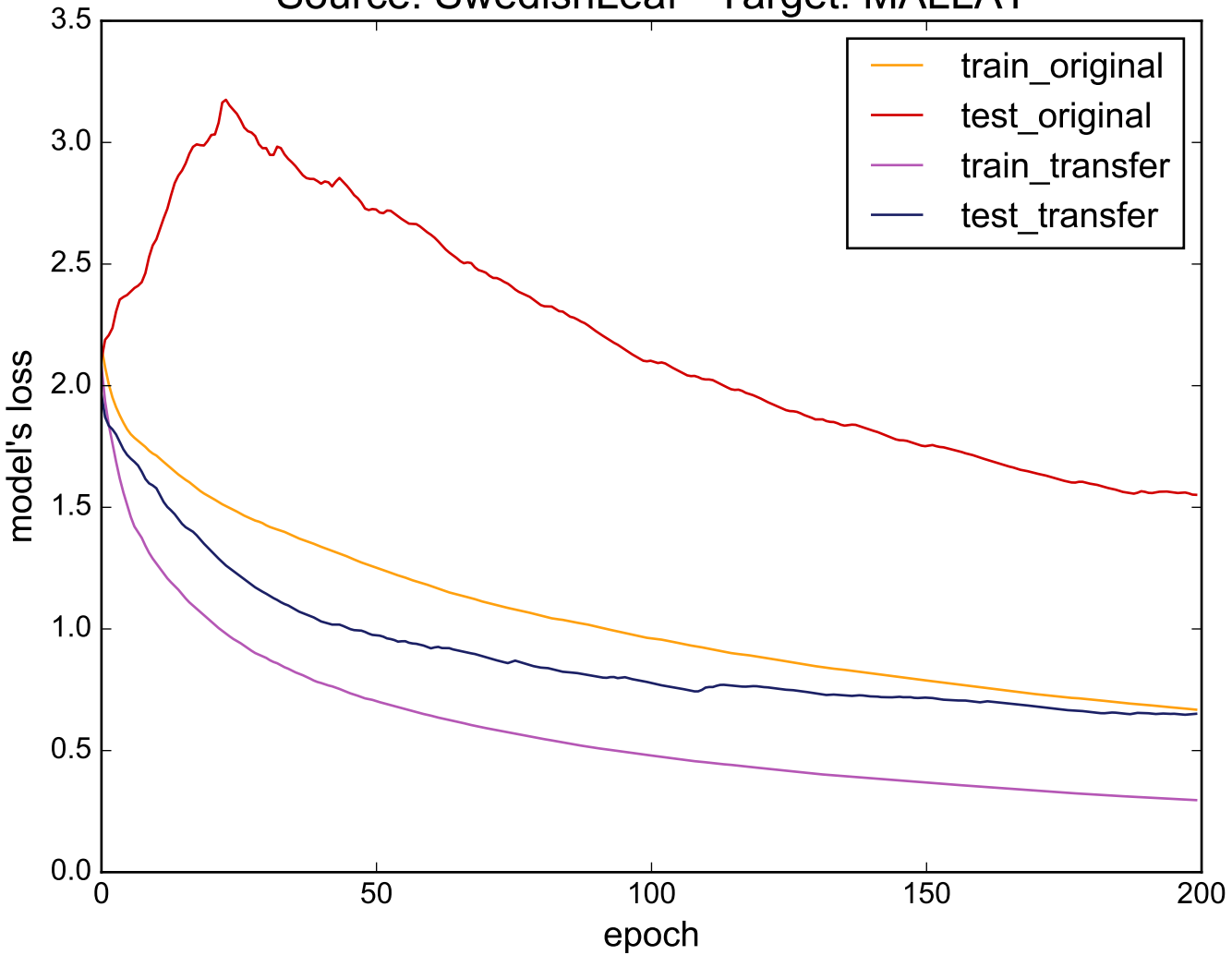
Source: SwedishLeaf - Target: MALLAT
