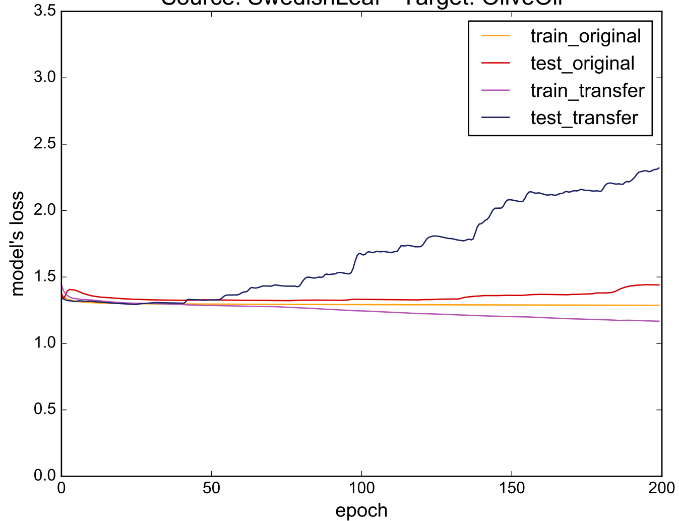
Source: SwedishLeaf - Target: OliveOil
