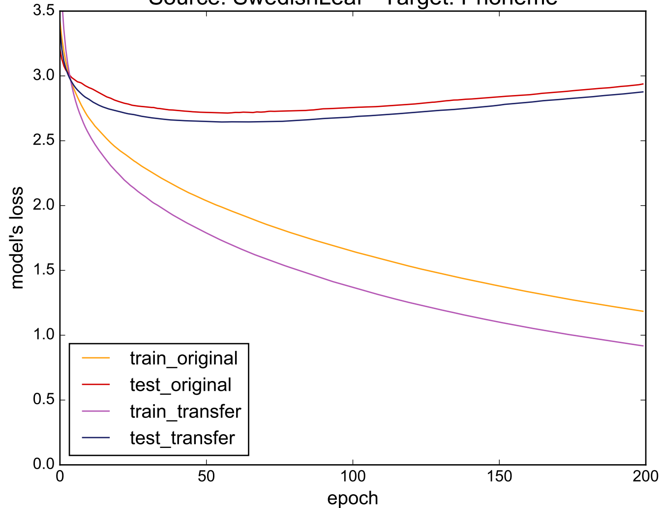
Source: SwedishLeaf - Target: Phoneme
