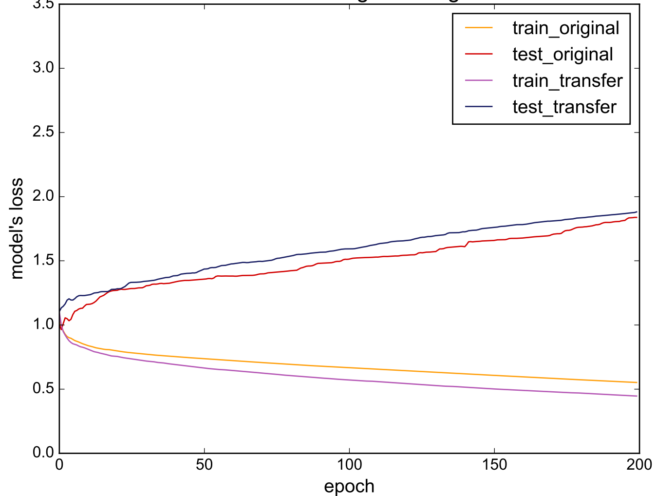
Source: SwedishLeaf - Target: RefrigerationDevices
