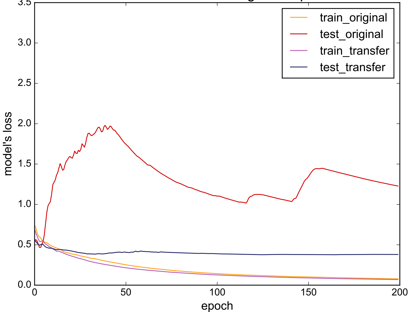
Source: SwedishLeaf - Target: ShapeletSim
