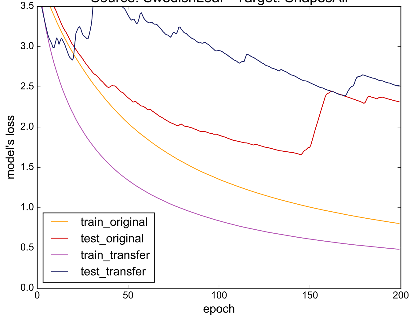
Source: SwedishLeaf - Target: ShapesAll
