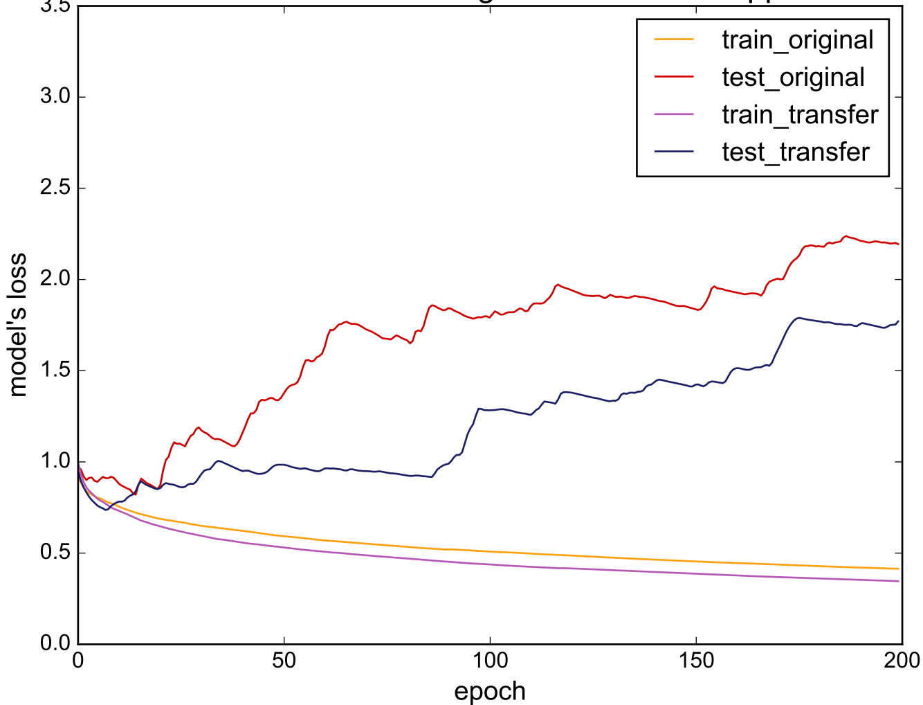
Source: SwedishLeaf - Target: SmallKitchenAppliances
