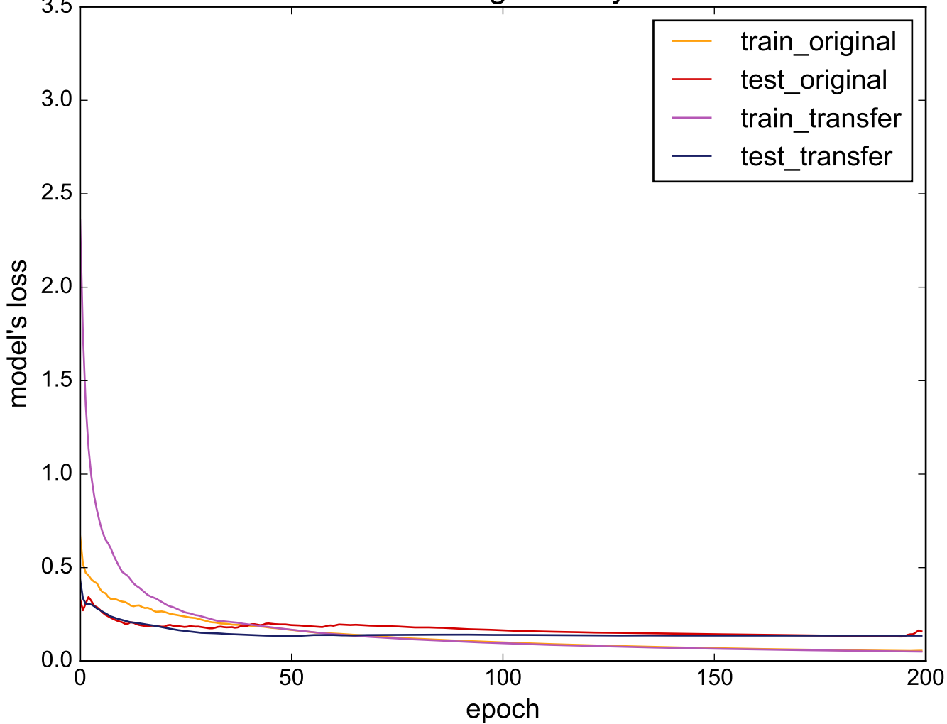
Source: SwedishLeaf - Target: SonyAIBORobotSurface
