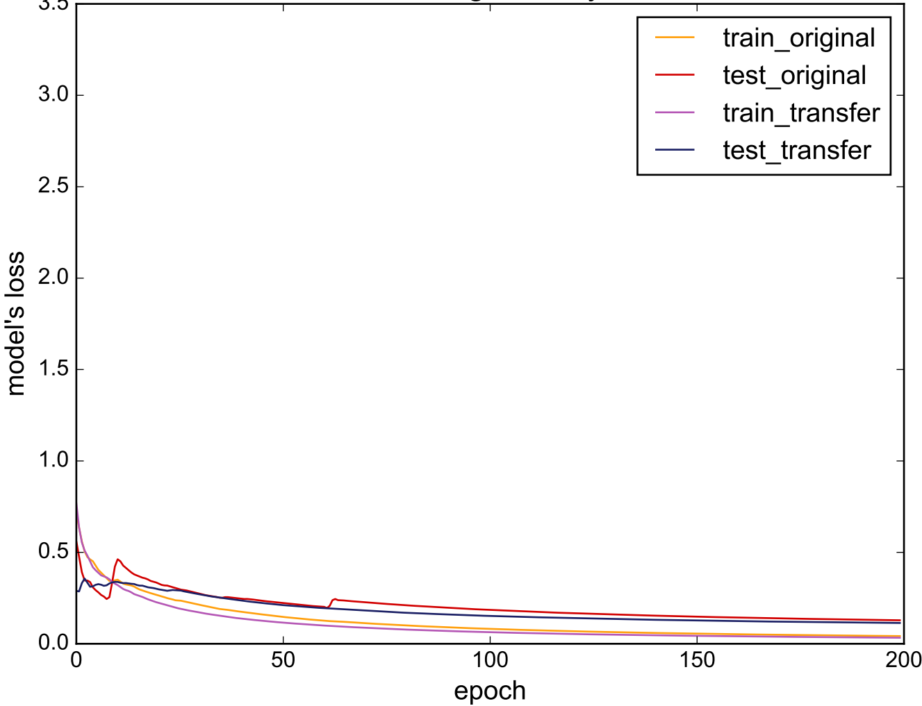
Source: SwedishLeaf - Target: SonyAIBORobotSurfacell
