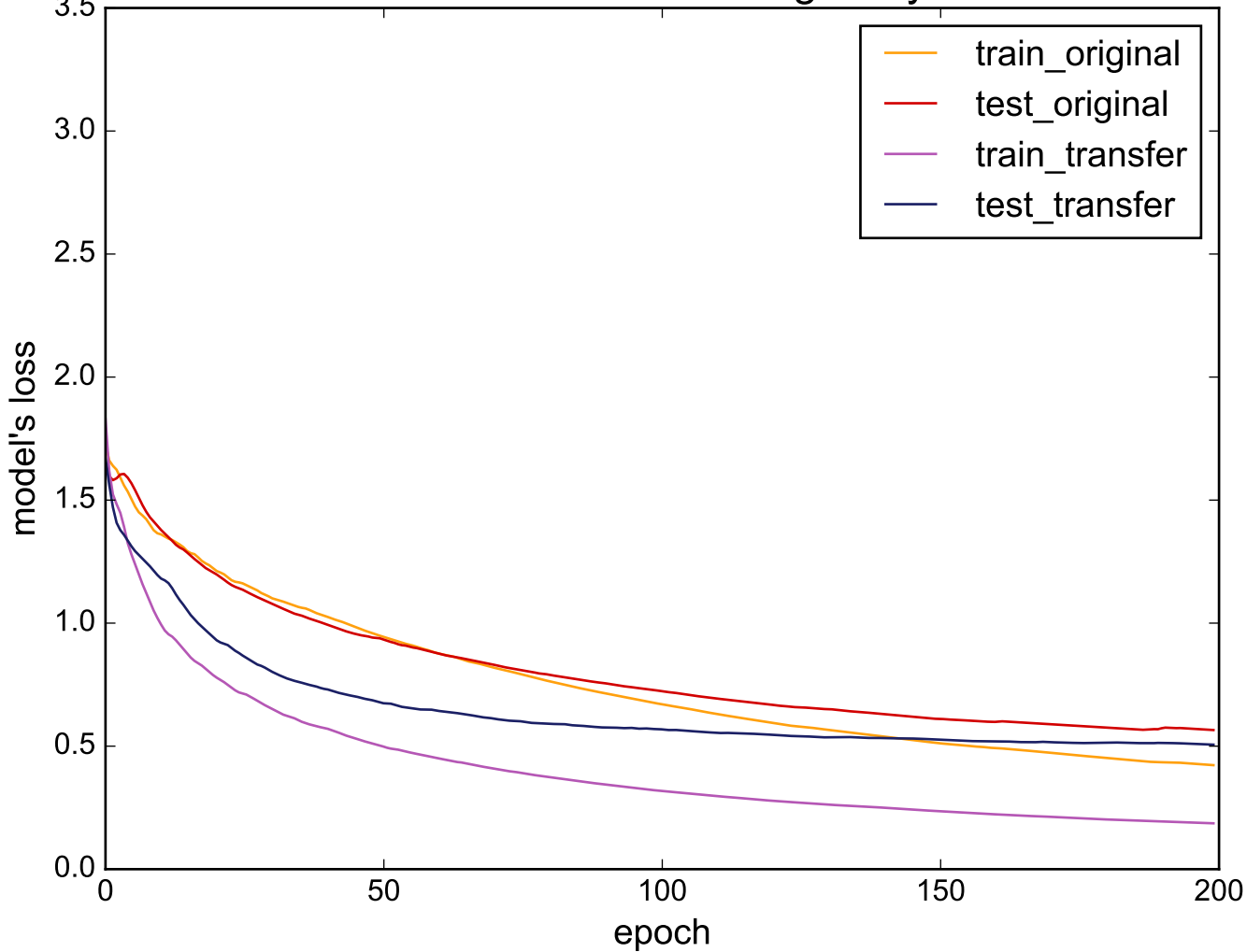
Source: SwedishLeaf - Target: Symbols
