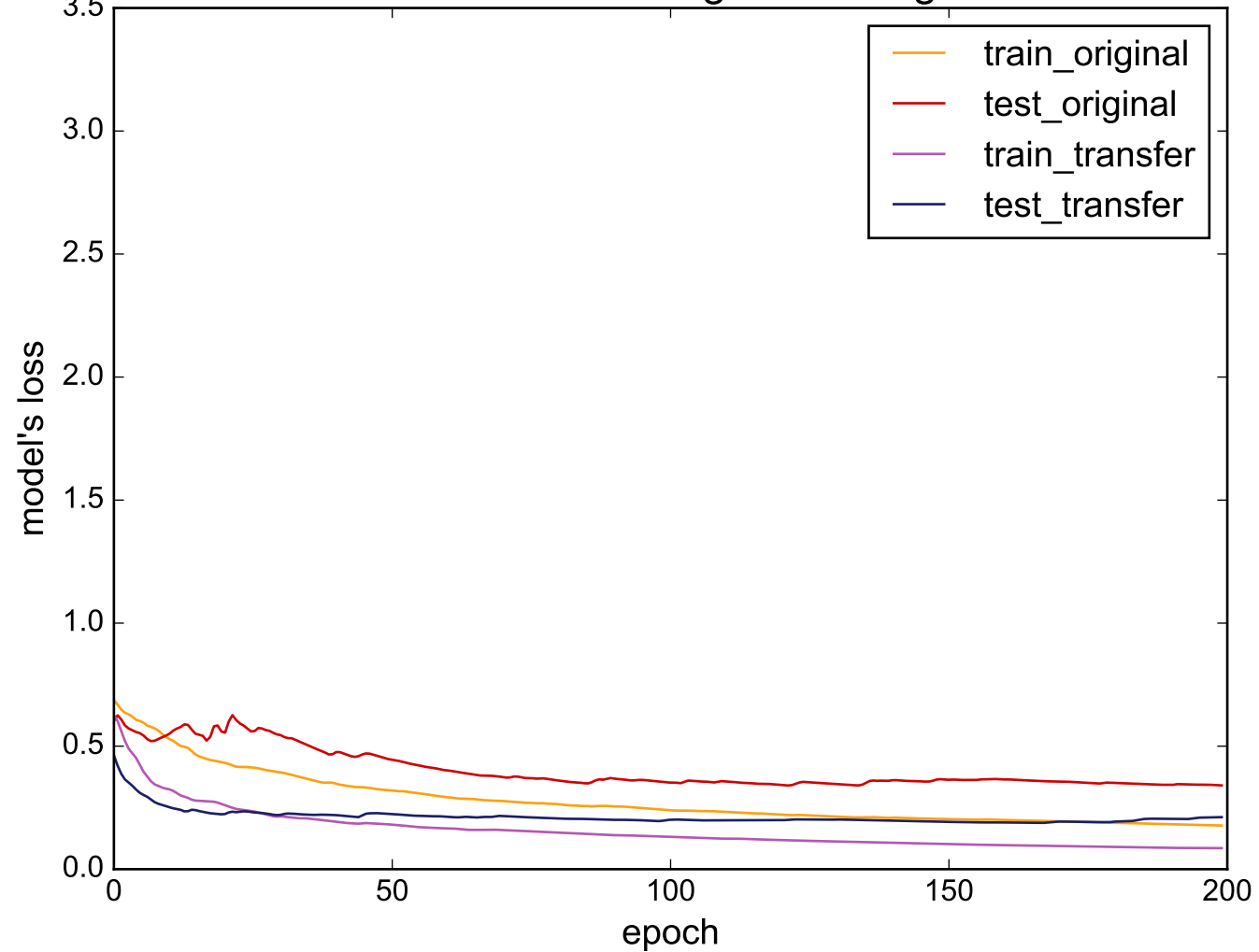
Source: SwedishLeaf - Target: ToeSegmentation1
