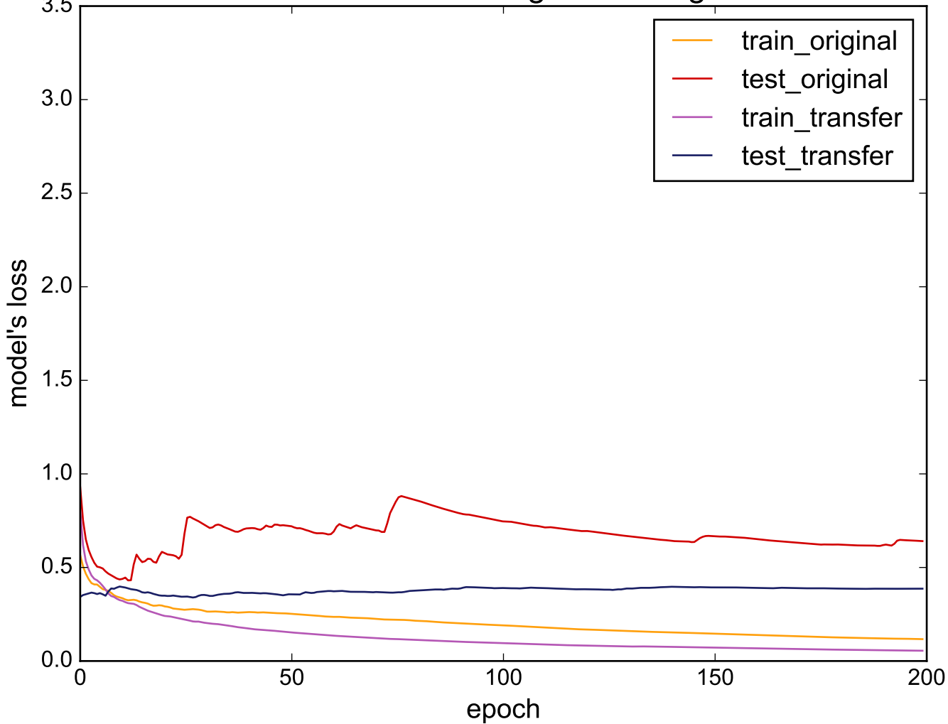
Source: SwedishLeaf - Target: ToeSegmentation2
