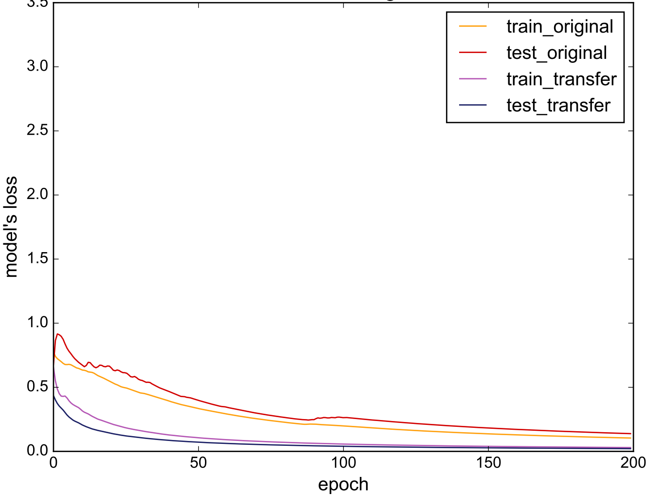
Source: SwedishLeaf - Target: TwoLeadECG
