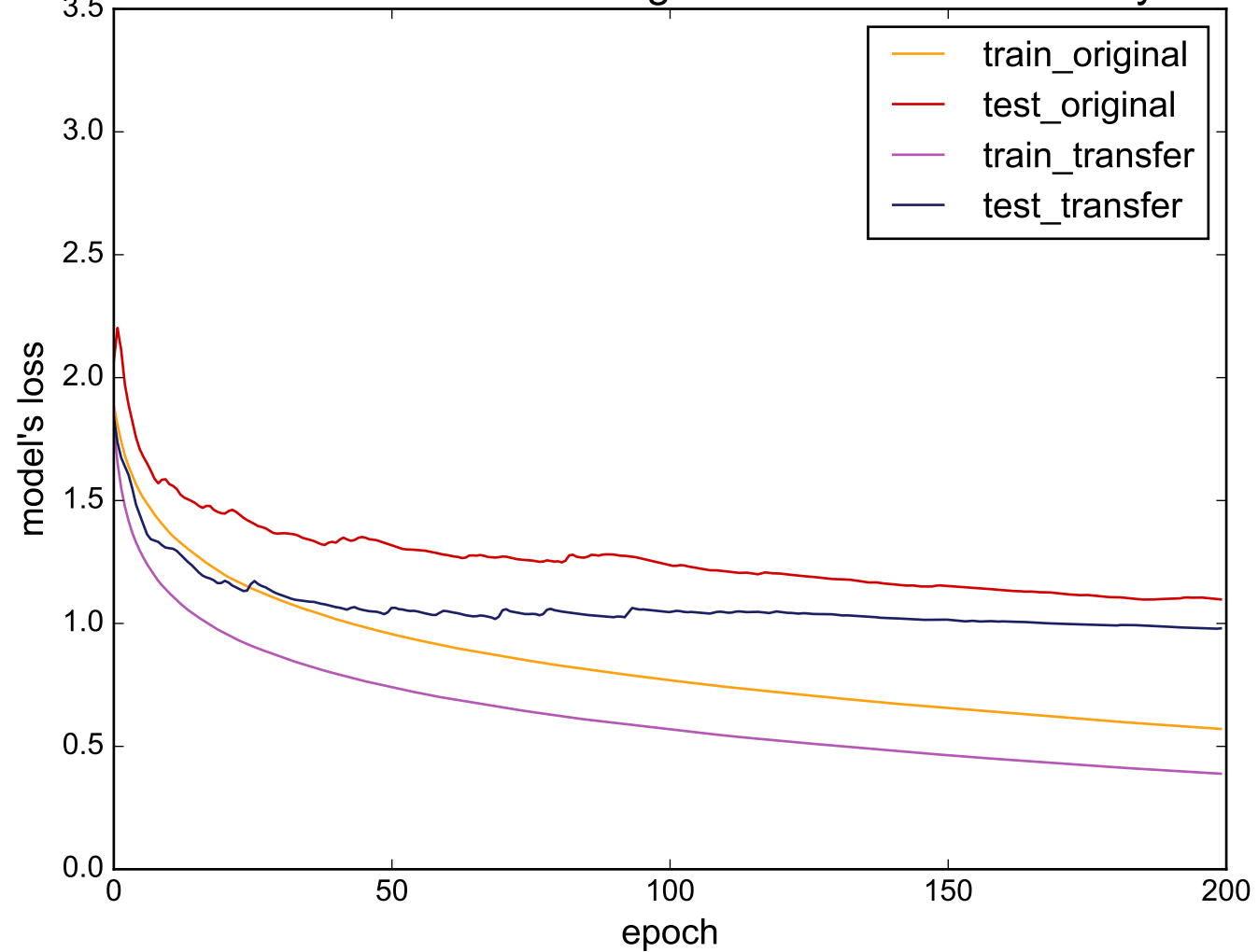
Source: SwedishLeaf - Target: UWaveGestureLibraryAll
