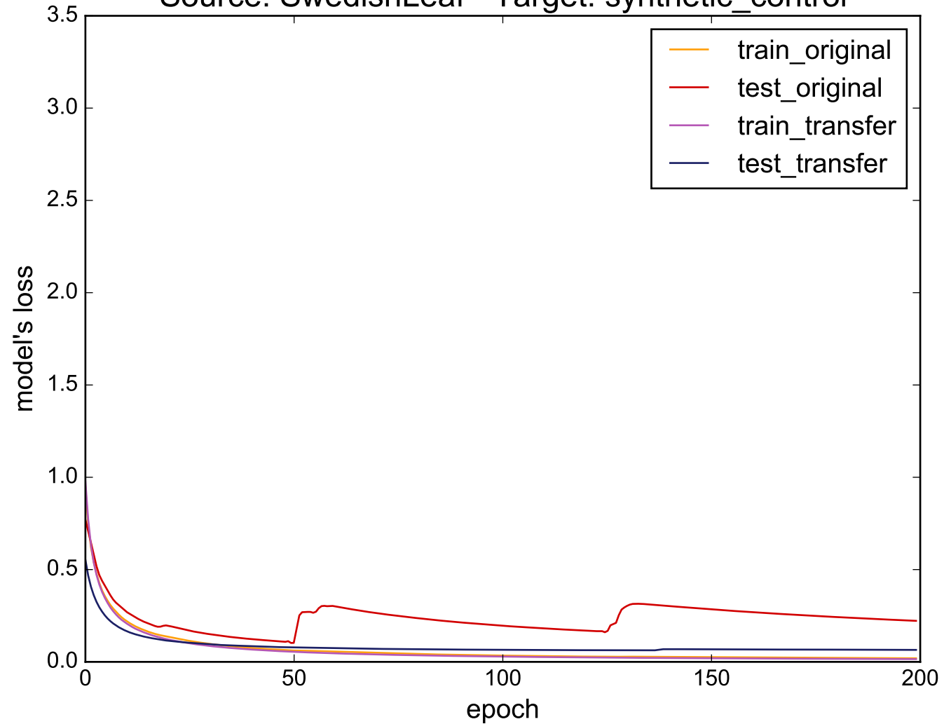
Source: SwedishLeaf - Target: synthetic_control
