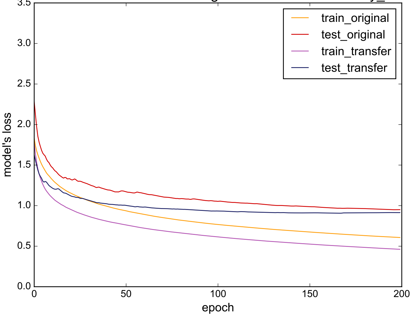
Source: SwedishLeaf - Target: uWaveGestureLibrary_X
