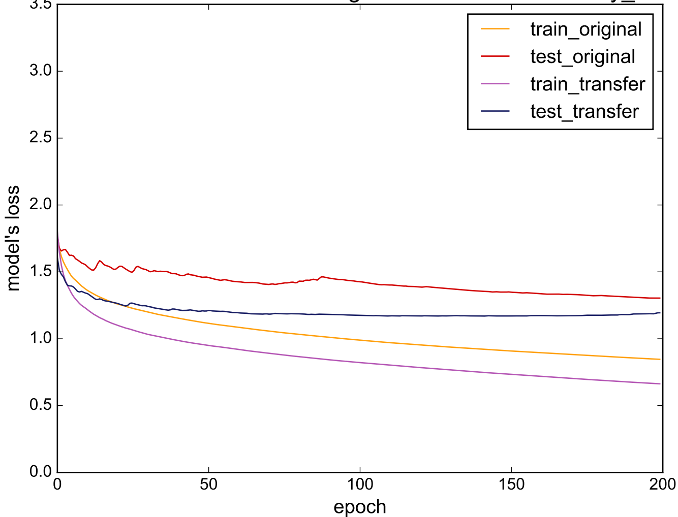
Source: SwedishLeaf - Target: uWaveGestureLibrary_Y
