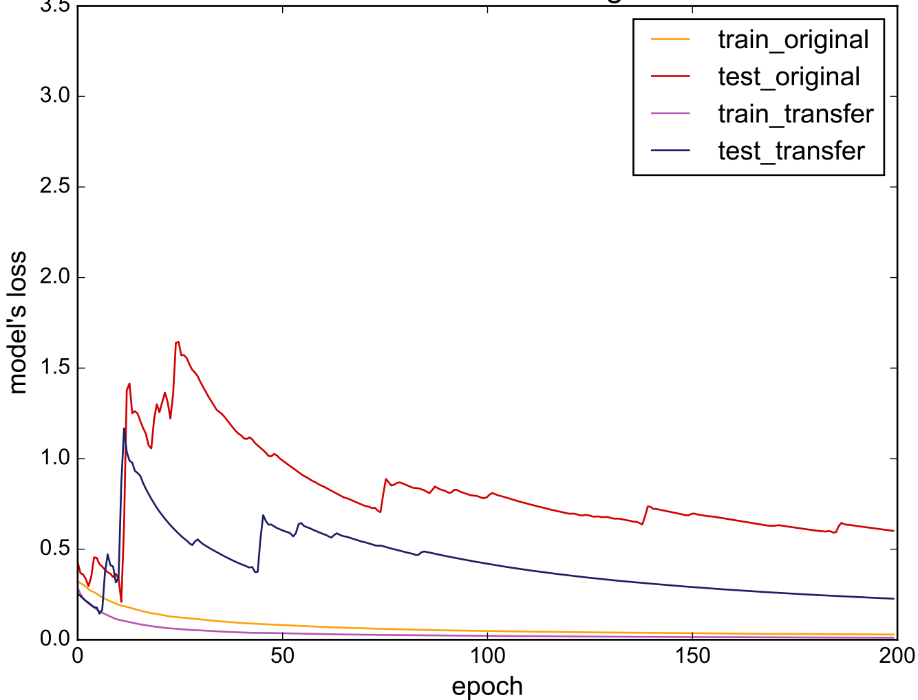
Source: SwedishLeaf - Target: wafer
